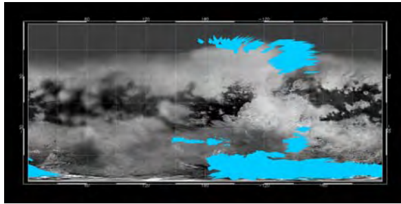
Figure 2. Global spatial distribution of clouds (in blue) in Titan's atmosphere as derived from all VIMS observations between October 2004 and July 2006.
