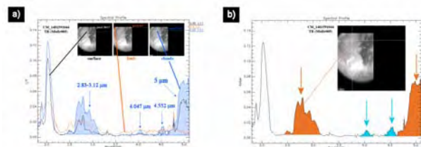
Figure 1. Left (a): Example of three very different Titan's spectra extracted from a single VIMS observation. Surface spectrum is in black, limb spectrum in orange and a typical "cloudy" pixel spectrum in blue. The "cloudy" spectrum is the only one to simultaneously present large atmospheric windows (in particular in the 3 and 5 \mu\text{m} spectral regions) and two small peaks at 4 and 4.5 \mu\text{m} , emerging from the noise in some cases. Right (b): Typical "cloudy" spectrum (same as the one showed in (a)) with an emphasis in blue and orange on spectral criteria applied by our automated cloud detection method.
