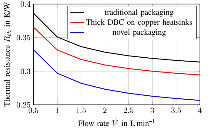
Fig. 9: Thermal resistance comparison between three possible packaging (simulation, jet impingement cooler with the same heat sinks (Design 4))
