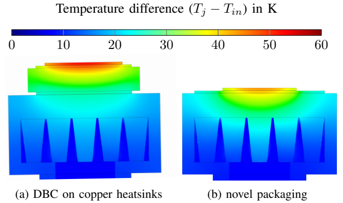
Fig. 8: Temperature distribution a traditional package which would provide the same electrical insulation as the novel packaging (same AlN thickness of 3\ \text{mm} ) and the novel packaging at 3\ \text{L}\ \text{min}^{-1}
