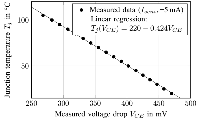
Fig. 12: Calibration the temperature-sensitive electrical parameter used for junction temperature monitoring: V_{CE} with 5 mA sense current and 9 V gate voltage.
