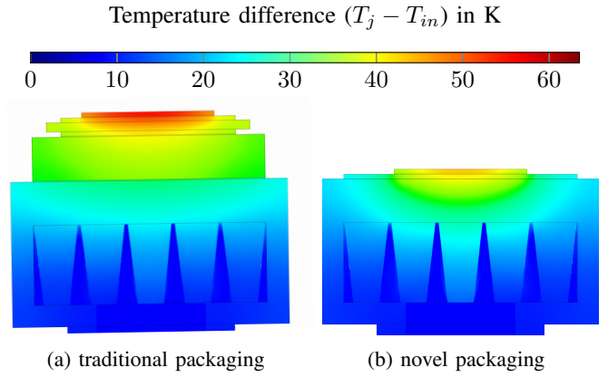
Fig. 7: Temperature distribution in the traditional and the novel packaging at 3\ \text{L}\ \text{min}^{-1}
