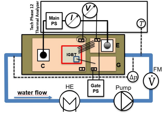
(c) schematic of the test setup
