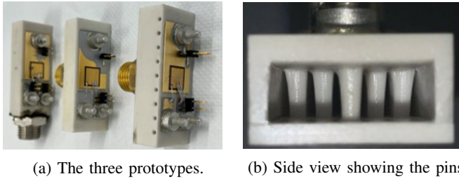
Fig. 10: The three prototypes: channel flow, jet impingement with two AlN thicknesses (1.5 mm and 3 mm);
