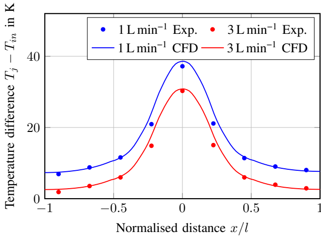
Fig. 14: Temperature distribution in the AlN for the jet cooler ( t = 3\text{mm} ), experiment ("Exp.") and simulation ("CFD").
