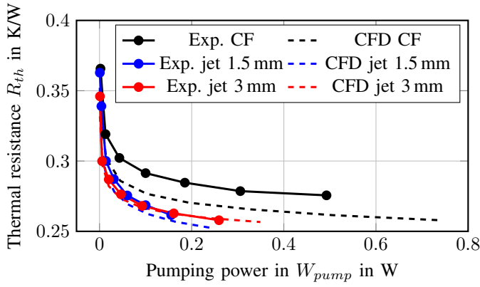
Fig. 13: Measured and simulated thermal resistances as a function of pumping power. "Exp.": experimental result; "CFD": simulation result; "CF": Channel flow configuration.
