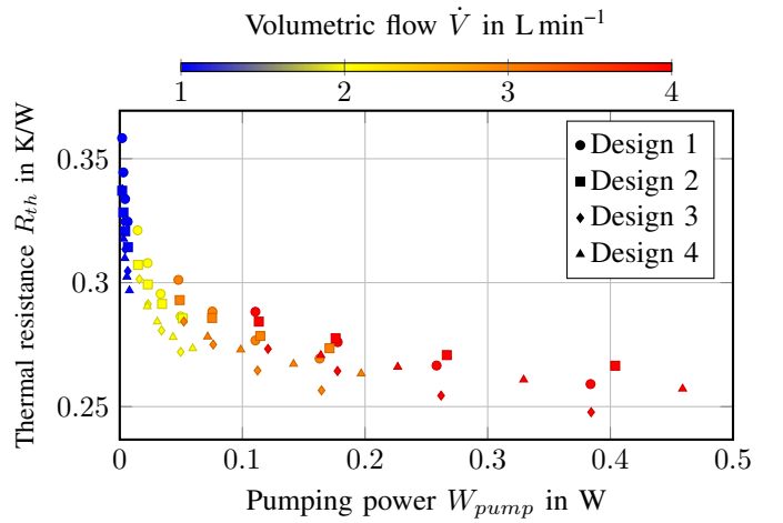
Fig. 3: Thermal resistance as a function of pumping power for all four jet impingement designs, color: flow rate
