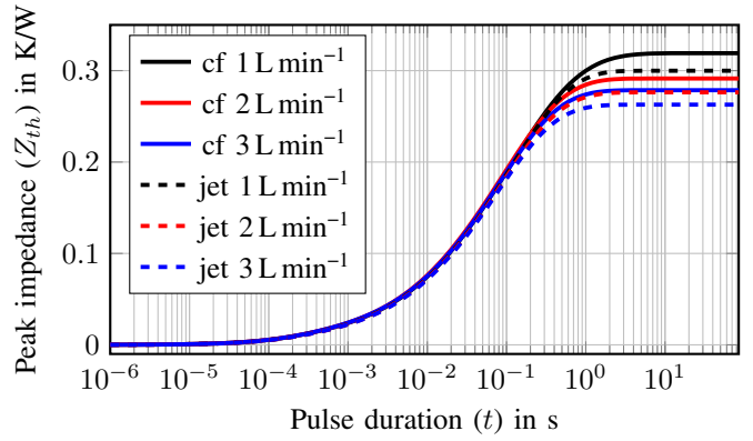
Fig. 15: Measured thermal impedance ( Z_{th} for two coolers and different flow-rates.
