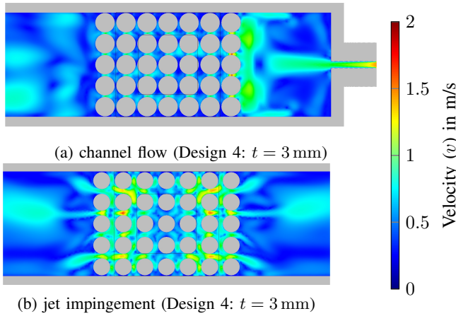
Fig. 6: Velocity distribution at 50\ \mu\text{m} distance from the upper wall under the chip at 3\ \text{L}\ \text{min}^{-1}
