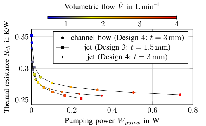
Fig. 5: Thermal resistance as a function of pumping power for different cooling concepts: channel flow and jet impingement (7.5 mm inlet diameter, AIN heatsinks).
