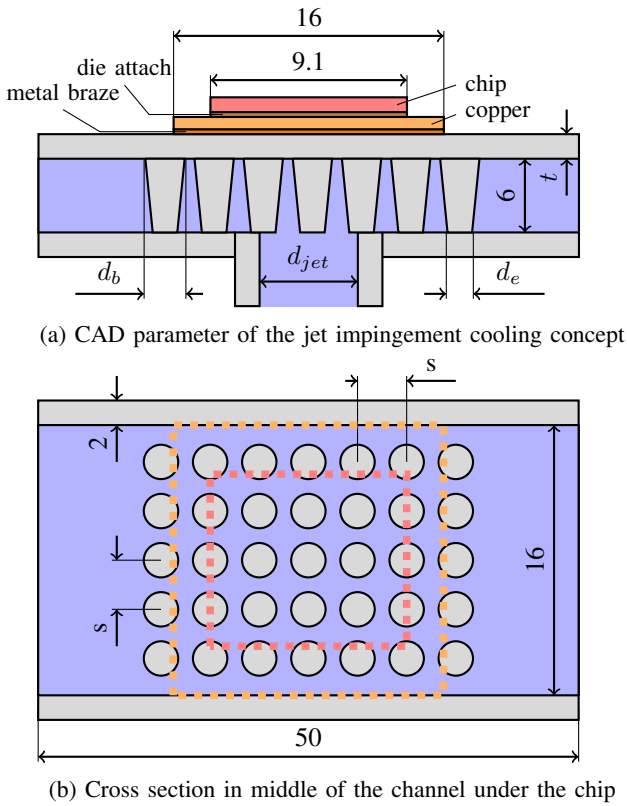
Fig. 2: Structure considered for the design, showing the design parameters
