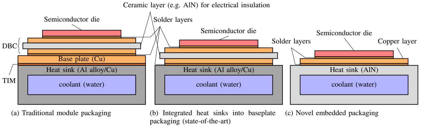
Fig. 1: Schematic comparison between the traditional, state-of-the-art and the novel power module packaging
