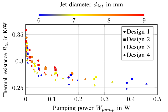
Fig. 4: Thermal resistance as a function of pumping power for all four jet impingement designs, color: jet diameter
