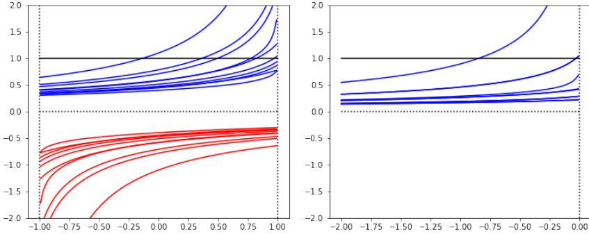
Figure 2. Birman-Schwinger principle. (Left). The spectrum of \lambda \mapsto K_V(\lambda) (Dirac case) for \lambda \in (-1, 1) , and V(x) = 2 \exp(-|x|^2/4) in dimension d = 2 . We only plotted the 10 largest (blue) and 10 lowest (red) eigenvalues. An energy \lambda is an eigenvalue of \mathcal{D}_m - V if one eigenvalue of K_V(\lambda) crosses the black line 1. (Right) Same for \lambda \mapsto \widetilde{K}_V(\lambda) (Schrödinger case) with \lambda \in (-2, 0) .
