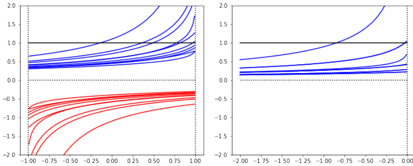
Figure 2. (Left). The spectrum of \lambda \mapsto K_V(\lambda) (Dirac case) for \lambda \in (-1, 1) , and V(x) = 2 \exp(-|x|^2/4) in dimension d = 2 . We only plotted the 10 largest (blue) and 10 lowest (red) eigenvalues. An energy \lambda is an eigenvalue of \mathcal{D}_m - V if one eigenvalue of K_V(\lambda) crosses the black line 1. (Right) Same for \lambda \mapsto \widetilde{K}_V(\lambda) (Schrödinger case) with \lambda \in (-2, 0) .
