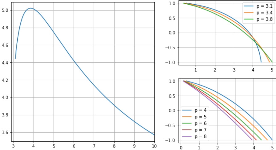
Figure 4. Radial case with d = 3 and m = 1 . (Left) The function p \mapsto \alpha_*^{\text{rad}, (\kappa=0)}(p) reaches its maximum at p \approx 3.86 . (Right) The maps \alpha \mapsto \Lambda_D^{\text{rad}, (\kappa=0)}(\alpha, p) for values of p corresponding either to p < 3.86 (top) or p > 3.86 (bottom).
