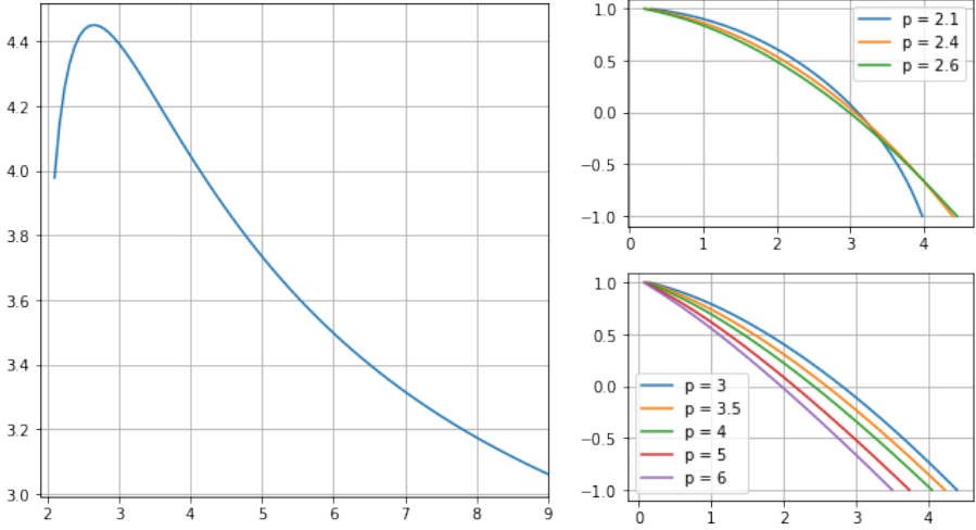
Figure 3. Radial case with d = 2 and m = 1 . (Left) The function p \mapsto \alpha_*^{\text{rad}, (n=0)}(p) is an upper bound for \alpha_*(p) and reaches its maximum for p \approx 2.66 . (Right) The maps \alpha \mapsto \Lambda_D^{\text{rad}, (n=0)}(\alpha, p) for values of p corresponding either to p < 2.66 (top) or p > 2.66 (bottom). Numerically the case n = -1 gives worse estimates.
