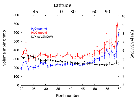
Figure 3: Volume mixing ratios of H 2 O (in ppmv, blue), HDO (in ppbv, red), inferred from the H 2 O/CO 2 and HDO/CO 2 line depth ratios corresponding to the transitions shown in Figure 1. The increase of these mixing ratios toward the south pole is consistent with the model predictions during southern summer (Ls = 304°). Black: the D/H ratio (in units of the VSMOW) inferred from the HDO/H 2 O line depth ratio. In all cases, the error bars are calculated from the dispersion of the six scans, and do not take into account the uncertainties associated with the radiative transfer model.
