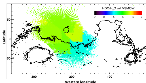
Figure 4: Map of the D/H ratio (in VSMOW units) inferred from the 1326-1338 cm -1 dataset of March 16, 2016.
