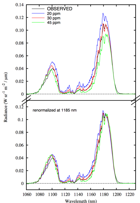
Figure 1: The SPICAV spectrum is compared to synthetic spectra calculated with H 2 O mole fractions of 20, 30 and 45 ppm using our best estimate for the representation of the H 2 O/HDO and CO 2 opacity. Upper panel : raw calculations; Lower panel : spectra renormalized to the observed radiance at 1185 nm.
