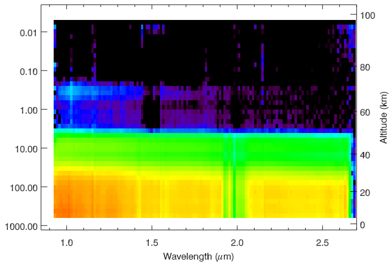
Figure 2: Figure 2: Optical thickness as a function of altitude and wavelengths for L_s = 343^\circ . The detached layer at 60 km presents the spectral signature of water ice at 1.5 \mu\text{m} .
