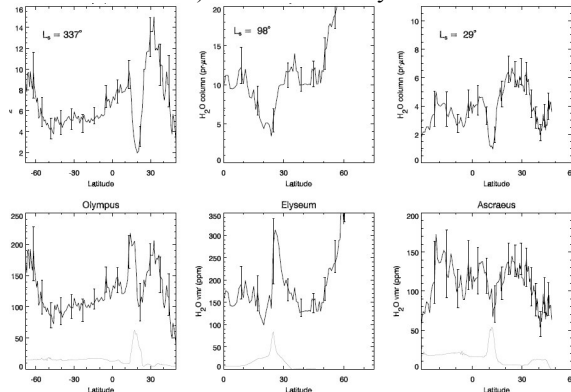
Figure 3. Absolute water columns and water volume mixing ratios below the saturation level (in part per million) in the region of three large volcanos. Olympus Mons (orbit 37), Elyseum Mons (orbit 925)
