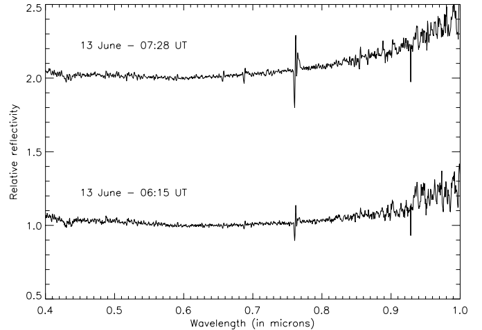
Fig. 3. Optical spectra of Chiron. The spectra have been normalized at 0.55 \mu\text{m} , and the upper spectrum has been shifted by 1 for clarity. The feature around 0.76 \mu\text{m} is due to bad correction of atmospheric features.
