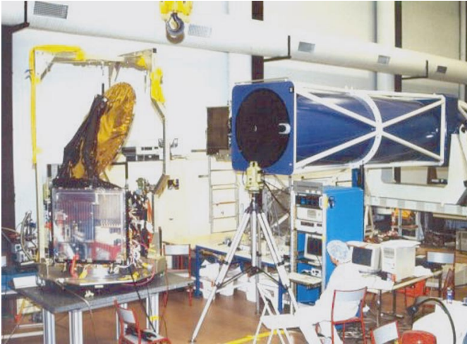
Fig. 5. The sub-mm collimator used for the alignment verification together with the Odin telescope with receiver platform during early tests. These were repeated after the launch simulation system tests just before launch.
