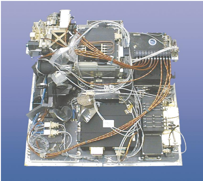
Fig. 4. The radiometer platform. From the front, on the left side is the autocorrelator with filterbank, pre-optics, Stirling cooler and LO structure. In the middle part is the cooler electronics with warm load, warm IF unit, PLL and control electronics, cryostat with biasing and, out of sight, the 119 GHz warm electronics. On the right is AOS, mechanism electronics and second autocorrelator.
