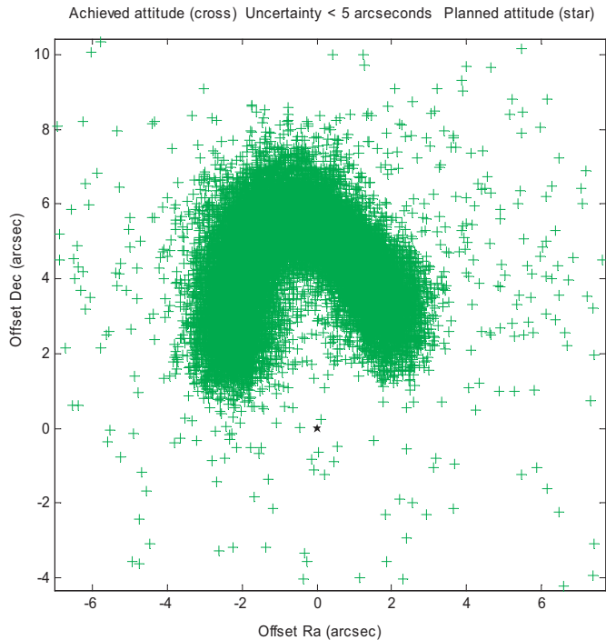
Fig. 6. Attitude error during several orbits. The position (0,0) is the target attitude. The points in this plot represent the attitude error at one sample ( dt = 1 s), projected in declination and right ascension. The half circle results from the uncorrected stellar aberration due to the spacecraft velocity around the earth.
