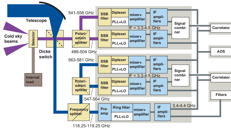
Fig. 1. This block diagram shows the layout of the instrument. High frequency signals from the telescope and the signal references are fed via pre-optics such as the Dicke switch, the single sideband filters and the diplexers for local oscillator injection, to the mixers. The mixers together with the first low noise amplifiers are mounted inside a cryostat. IF signals are after further amplification routed to the backend spectrometers.
