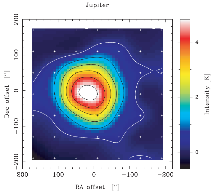
Fig. 7. Jupiter map at 557 GHz. The mapping, at 60'' spacing, was performed in the position-switching mode, using a reference off at +1800'' in RA. The crosses denote map positions in our re-gridded map (best-fit after attitude reconstruction).
