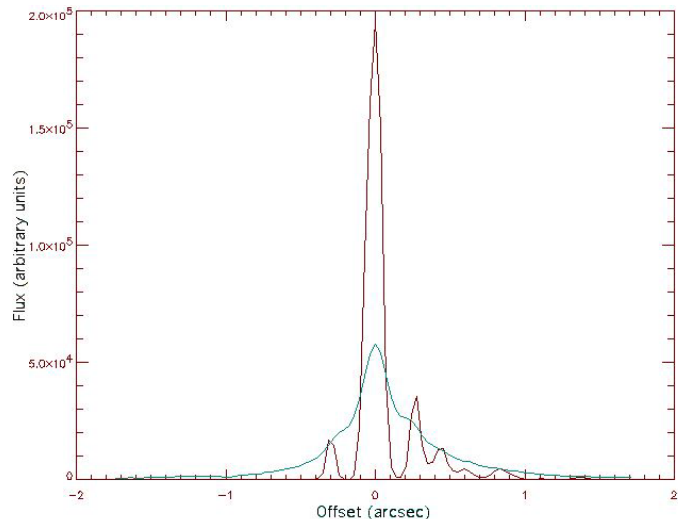
Fig. 2. Deconvolved light profile (black) of NGC 1068. The undeconvolved profile is plotted in grey.
