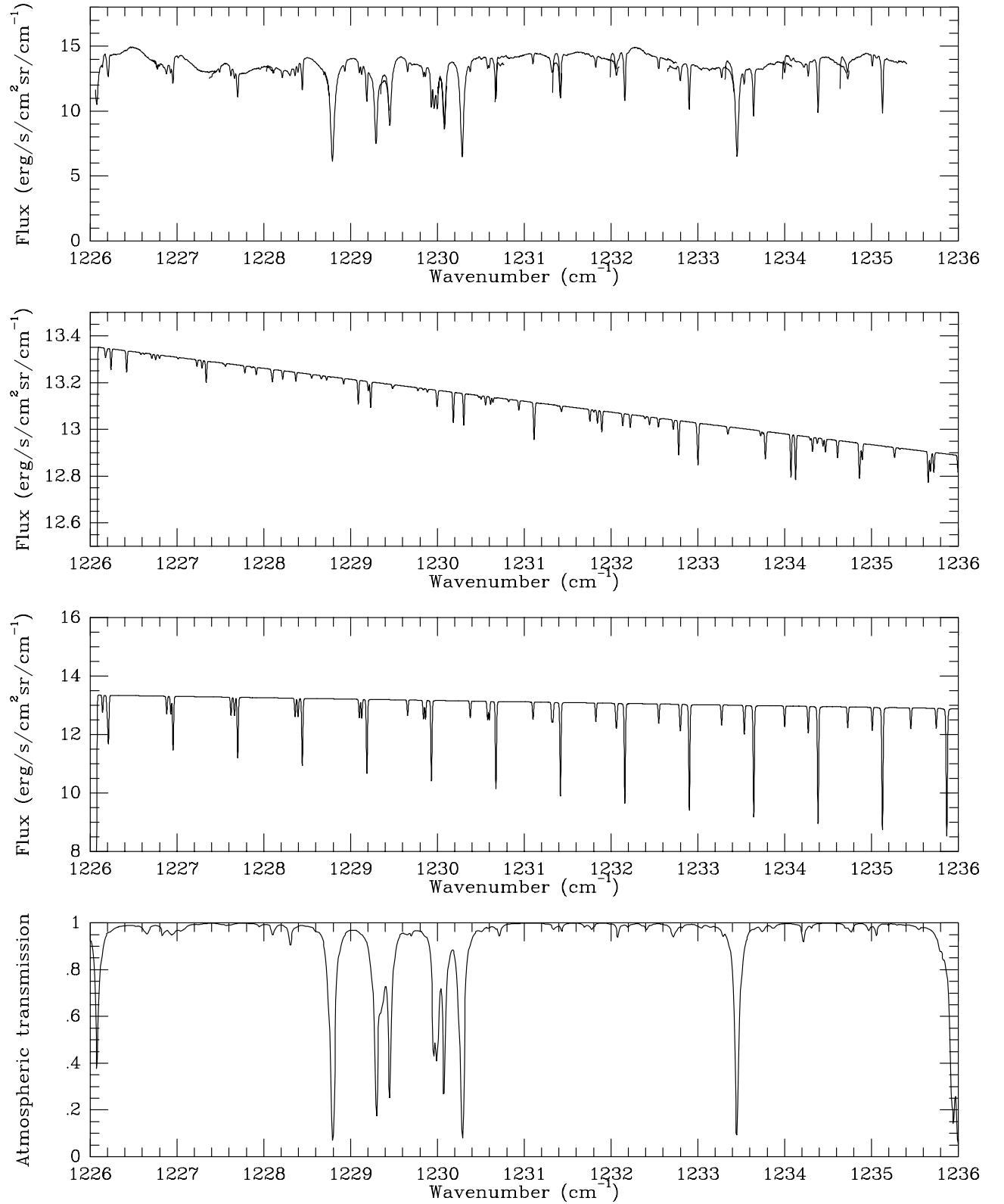
Fig. 2. From top to bottom: a) The spectrum of Mars at low northern latitudes (10N–40N) between 1226 and 1236 \text{cm}^{-1} (spectrum S1). The spectral resolution is 0.017 \text{cm}^{-1} . b) A synthetic spectrum of H 2 O 2 under the Martian conditions (see Sect. 3), corresponding to a column density of 2 \times 10^{16} \text{ cm}^{-2} (mean mixing ratio of 10^{-7} ). c) A synthetic spectrum of CO 2 under the Martian conditions. d) A synthetic model of the terrestrial atmospheric transmission at Mauna Kea, for a terrestrial water content of 1 pr-mm and a zenith angle of 45 deg. The Mars spectrum is dominated by Martian CO 2 and incompletely cancelled telluric CH 4 , in addition to broad features due to imperfect flat-fielding.
