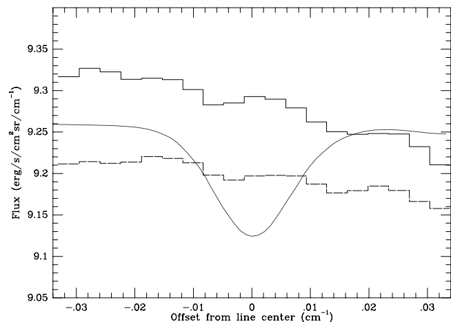
Fig. 5. The S2 and S4 spectra of Mars of Feb. 3, 01 (histograms) co-added in 6 spectral intervals of 0.07 cm -1 each, centered on H 2 O 2 line frequencies (see text). Solid line: S4 (40N–60N); long-dashed line: S2 (0–90N). Dotted line: the corresponding synthetic spectrum calculated with H 2 O 2 only, shifted by 0.072 cm -1 (H 2 O 2 column density of 2 \times 10^{16} cm -2 , corresponding to a mean mixing ratio of 10^{-7} ). The spectral resolution is 0.017 cm -1 .
