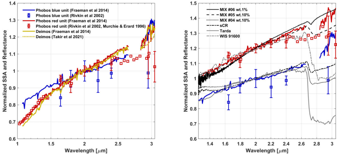
Figure 5. Left-hand panel, selection of ground-based and spacecraft data of Phobos (both red and blue units) and Deimos. All spectra are normalized at 2 \mu\text{m} in order to show differences in slope that characterize the two spectral types observed on the moons. All the spectra show a good agreement considering the large error bars of some ground-based observations. Right-hand panel, comparison between selected spectra of Phobos and laboratory analogues. Spectra of the red unit and blue unit are normalized at 2 \mu\text{m} and offset for clarity. We compared the mixture (black lines) and meteorites (grey lines), showing the best match with the observation. Although the agreement with the slope is pretty good in the studied range, the comparison in the region of the 2.7 \mu\text{m} hydrated band is of lower quality due to both the worse quality of the Phobos spectra and the more intense bands of some laboratory spectra.
