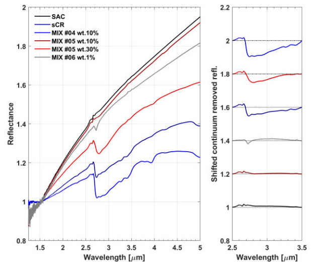
Figure 3. Left-hand panel, best analogue laboratory spectra for matching Phobos and Deimos in the NIR range. In detail: synthetic amorphous carbon (SAC), mixture of sCR with sMARS in 10 wt. per cent (MIX #04), SAC mixed with basaltic mixture, 50/50 bytownite and augite (MIX #05) in 10 wt. per cent, and 30 per cent of the basalt component and SAC mixed with serpentine at 1 wt. per cent. Right-hand panel, details of hydrated band at about 2.7 μm of spectra in left-hand panel after continuum removed and offset for clarity.
