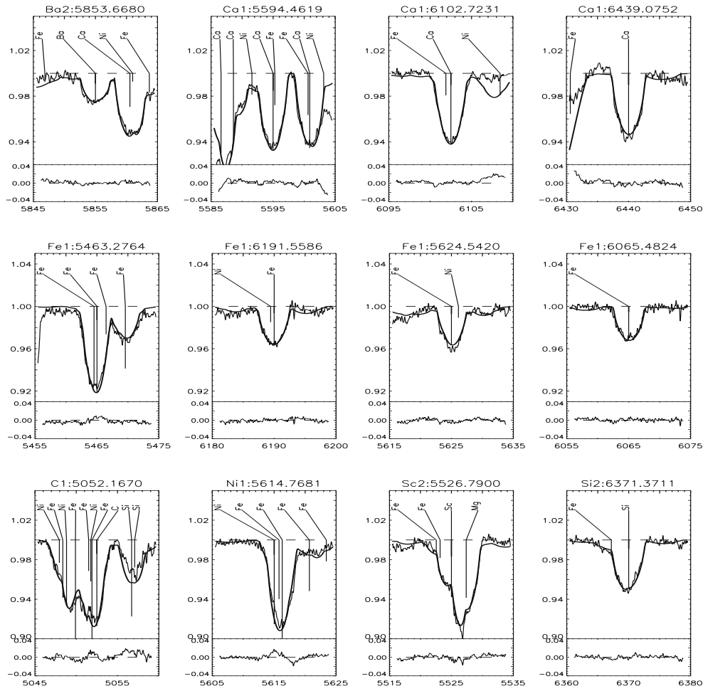
Fig. 1. Observed (thin line) and synthetic (thick line) spectrum around twelve lines which were used for the abundance determination. The lower portion of the each plotted line shows the relative difference between the observed and synthetic spectrum. The name of the element and the central wavelength (in Ångström) of each fitted line is given at the top of each plot.
