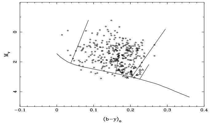
Fig. 4. Location of HD 49434 (star symbol) in the HR diagram together with the known \delta Scuti (circles, Rodríguez & Breger 2001) and bona fide \gamma Dor (triangles, Handler & Kaye 2001) pulsators. The edges of the \gamma Dor region around (b - y)_0 = 0.2 are from Handler (1999). The absolute magnitude of HD 49434 is M_V = 2.73 \pm 0.07 and is derived from its Hipparcos parallax (ESA 1997).
