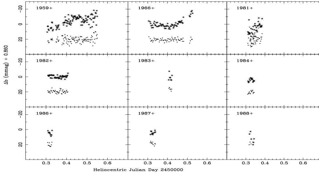
Fig. 2. Differential magnitudes of HD 49434 minus comparison star HD 48922 in the Strömgren b band (asterisks). The dots are the magnitude differences between the two comparison stars HD 49933 and HD 48922 (shifted to allow comparison). Individual days are marked in every panel as the corresponding HJD.
