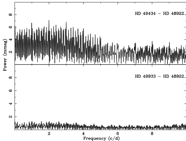
Fig. 3. Power spectra corresponding to the variable star HD 49434 minus the comparison star HD 48922, in the upper panel, and that corresponding to the comparison stars HD 49933 minus HD 48922 in the bottom panel. The scales are milli-magnitudes and cycles/day.
