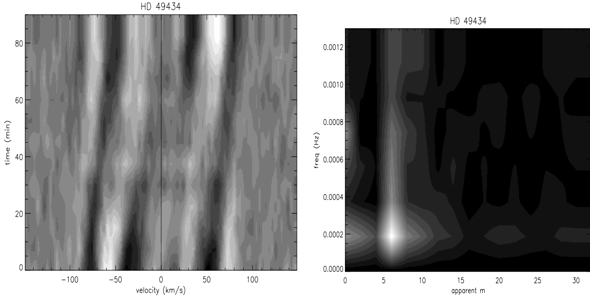
Fig. 5. The residual of the mean profile for the January 2000 series. Left: in velocity – time space; the maximum amplitude is of the order of 3 \times 10^{-3} ; Right: Spectral power density of the same data, in apparent order – frequency space, after the 2D Fourier transform.
