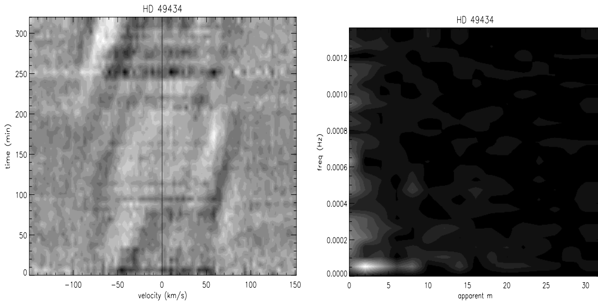
Fig. 6. The same as Fig. 5 but for the December 2000 series; the maximum amplitude of the residuals is of the order of 4 \times 10^{-3} .
