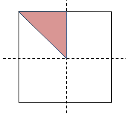
Figure 9: The calculated part (in red) of a square borehole field after symmetry simplification
