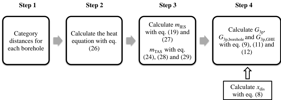
Figure 13: The flow chat of the global model for fast calculation of the thermal response factors
