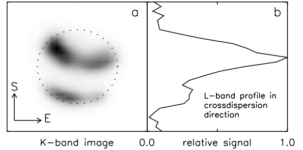
Fig. 1. a) ISAAC K -band target acquisition image of Neptune. The dotted circle has a diameter of 2.35'' . b) Relative signal profile in cross-dispersion direction during spectral L -band observation.
