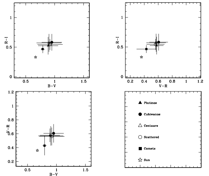
Fig. 4. Color-color diagrams of the average populations
