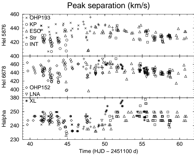
Fig. 12. Variations in \text{km s}^{-1} of the emission peak separation of the He I 5876, 6678 and H\alpha lines during the MuSiCoS 98 campaign.
