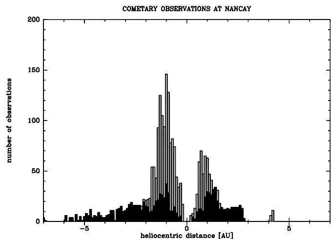
Fig. 5. Distribution of the observations as a function of heliocentric distance (negative: pre-perihelion; positive: post-perihelion).
