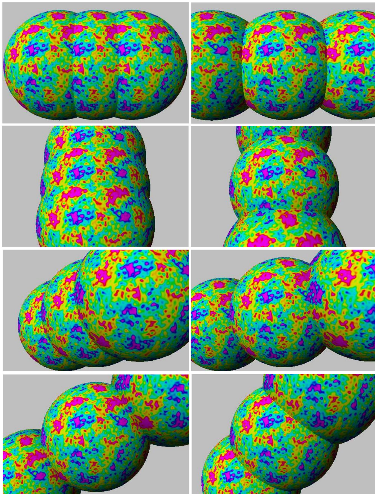
FIG. 8. (Color online) Eight pairs of matching circles among the 61 existing pairs for a single realization of the density fields. For clarity, the orientation of the last scattering surface is the same in all panels.
