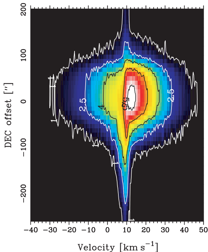
Fig. 3. H 2 O declination-velocity diagram through Orion KL. The colour coding goes from black ( \leq 1 K), to white ( \geq 7 K). The contours 2 start at 1 K and are incremented with 1.5 K.
