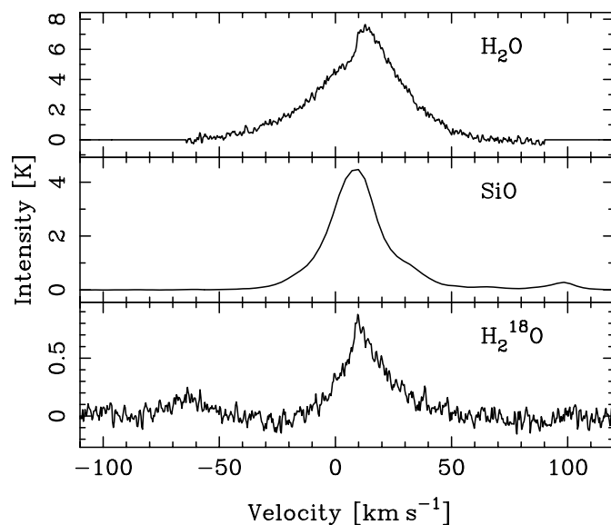
Fig. 4. From top to bottom: H 2 O (Odin beam 2.1'), SiO (Onsala; beam size 0.7'), and (Odin) H 2 18 O (accompanied by an SO 2 emission line at \sim -60 km s -1 , see text). Note the different vertical scales 2 .
