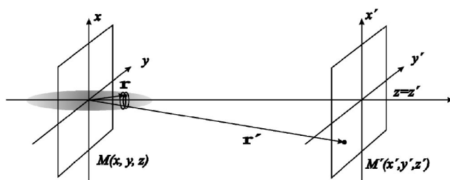
FIG. 2. Huygens-Fresnel propagation used in the model.
