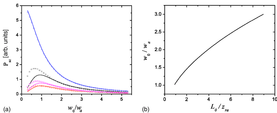
FIG. 6. (Color online) (a) Scattered power vs relative size of sample and probe beam for samples ( w_a=10\ \mu\text{m} ) of length L_0=1, 400, 738, 1000\ \mu\text{m} (diamonds, squares, stars, triangles) together with the analytic prediction from Eq. (14) (solid lines) in scaled units; (b) predicted probe beam size to match input and scattered wave as a function of sample length in scaled units.
