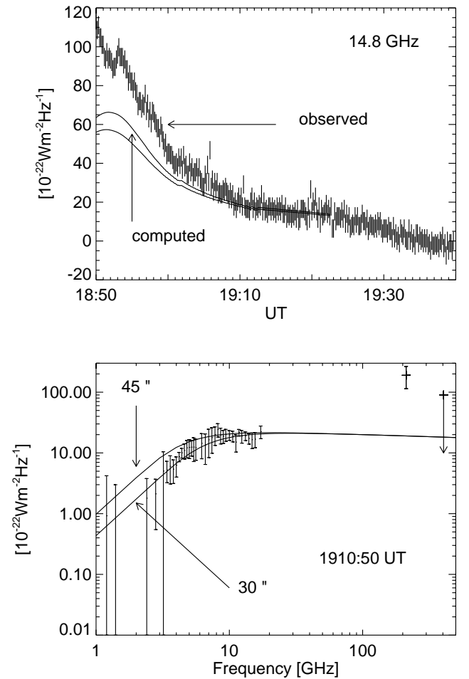
Fig. 5. Top panel: time evolution of the 14.8 GHz flux density observed by OVSA during the decay of the microwave emission and computed for a 30'' and a 45'' isothermal source, the emission measure and temperature of which have been derived from the GOES SXR observations. Bottom panel: observed (error bars) and computed (solid line) radio spectra when the microwave emission is predominantly produced by free-free emission.
