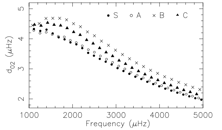
Fig. 4. Small separations d_{02} for all 4 models.
