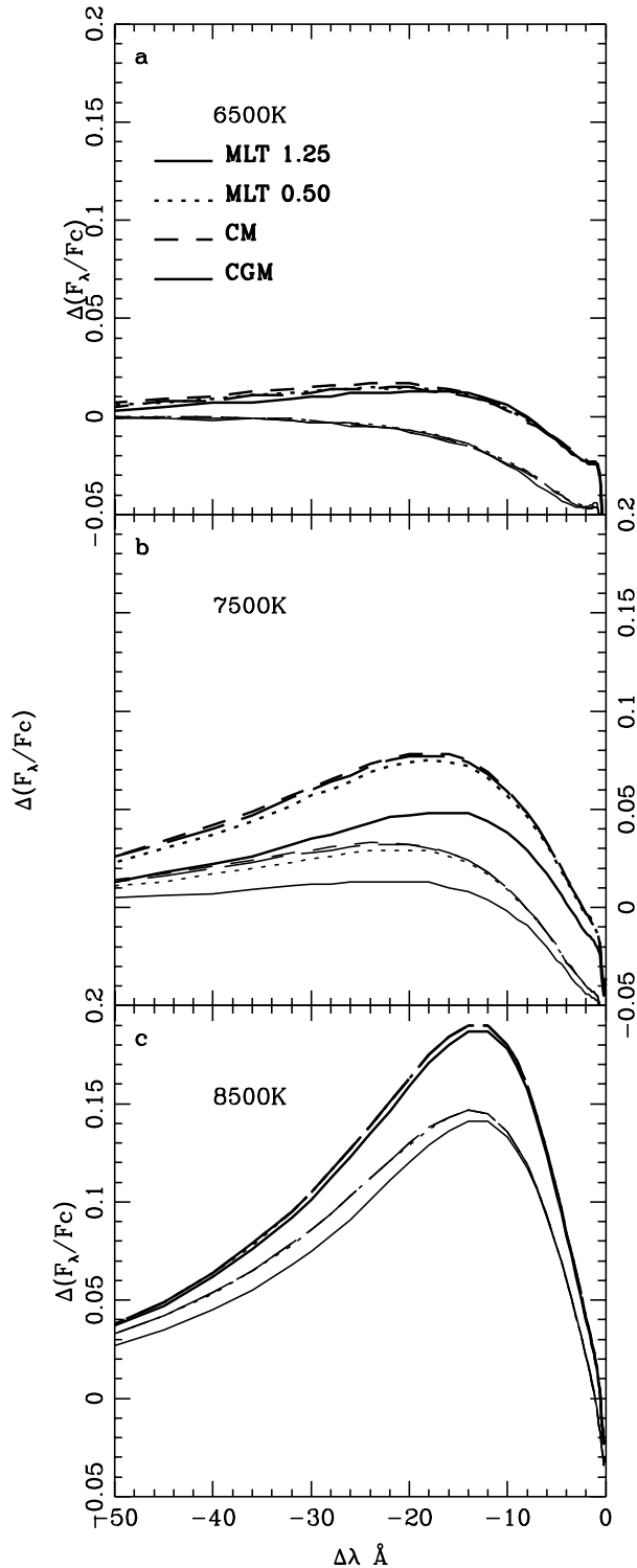
Fig. 7. Differences between H_\beta line profiles computed with \log g = 2.5 and 4.5 . Different convection models are represented by different line styles, for metallicities of -1 and +1 by thin and thick lines respectively, and for three effective temperatures.
