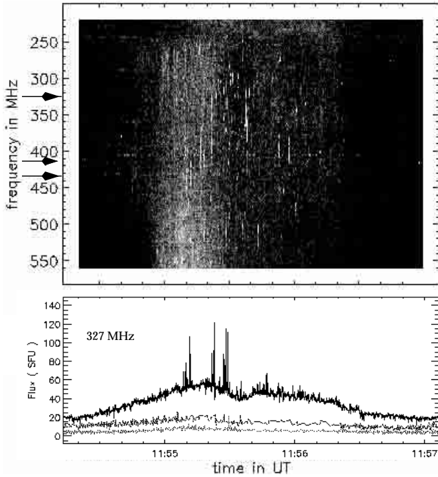
Fig. 1. Top: spectrogram observed by Phoenix-2 on 2000/07/12. Bright pixels correspond to enhanced flux; the frequency axis is from top to bottom. The arrows indicate the frequencies observed by NRH. Bottom: NRH light curves at 327 MHz of the three major sources present on the solar disk.
