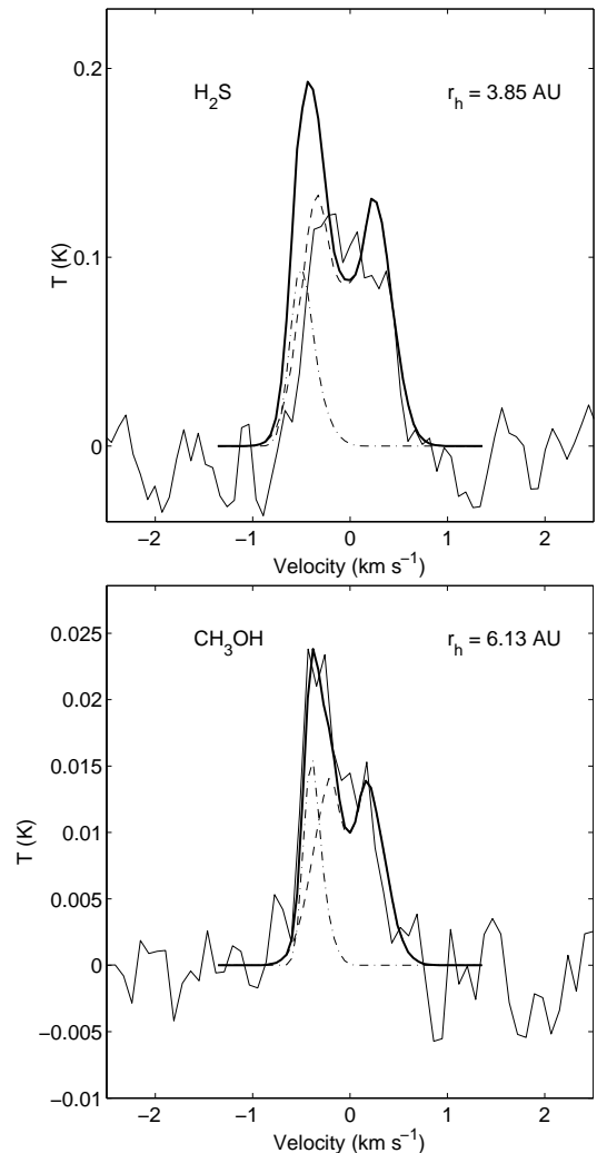
Fig. 9. Observed emissions (thin lines) for the \text{H}_2\text{S } 1_{10-1_{01}} line (top) and the \text{CH}_3\text{OH } 3_{0-2_0} A^+ line (bottom) compared to the modeled CO J(2-1) lines from the two components in the extended source case. The nuclear and extended components are dash-dotted and dashed lines, respectively. The thick line is the composite modeled CO line. The model line is divided by 2 in the bottom figure.
