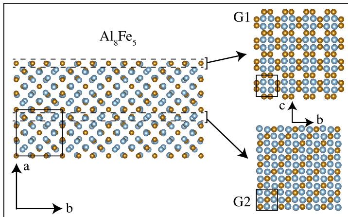
Figure 3: Left) \text{Al}_8\text{Fe}_5 bulk structure viewed along the [001] direction. Right) Two different types of (100) planes referred as G1 and G2 are present within the bulk model. The Al and Fe atoms are represented as light blue and brown spheres respectively.
