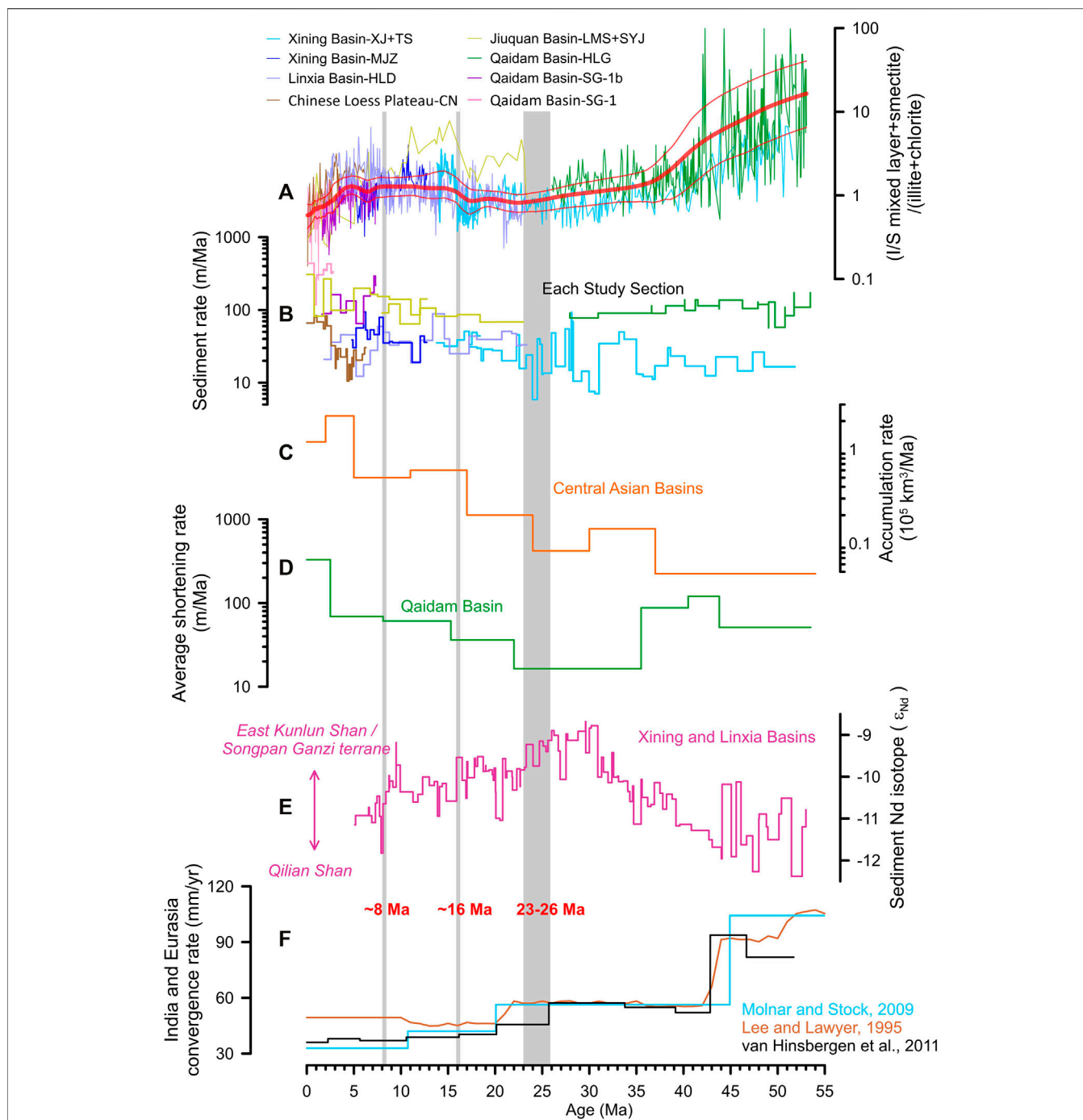
FIGURE 2 | Cenozoic silicate weathering history in the NE Tibetan Plateau and its comparison with provenance, erosion and tectonic records (A) Compiled (I/S mixed layer + smectite)/(illite + chlorite) ratio (B) Sedimentation rates of the study sections (Xining Basin: XJ section, Dai et al., 2006; TS core, Zan et al., 2015; MJZ section, Yang et al., 2017; Qaidam Basin: SG-1 core, Zhang et al., 2012; SG-1b core, Zhang et al., 2014; HLG section, Fang et al., 2019b; Linxia Basin: HLD section and HZ core, Fang et al., 2016; Jiuquan Basin: LJM section, Fang et al., 2005; SYJ section, Song, 2006; Chinese Loess Plateau: CN section, Song et al., 2001) (C) Average accumulation rate in Central Asian basins (Métivier et al., 1999) (D) Average shortening rate in the Qaidam Basin (Bao et al., 2017) (E) Nd isotope of decarbonated bulk sediments from the Xining and Linxia Basins (He et al., 2019; Yang et al., 2021a) (F) Convergence rates between India and Eurasia (Lee and Lawyer, 1995; Molnar and Stock, 2009; van Hinsbergen et al., 2011).
