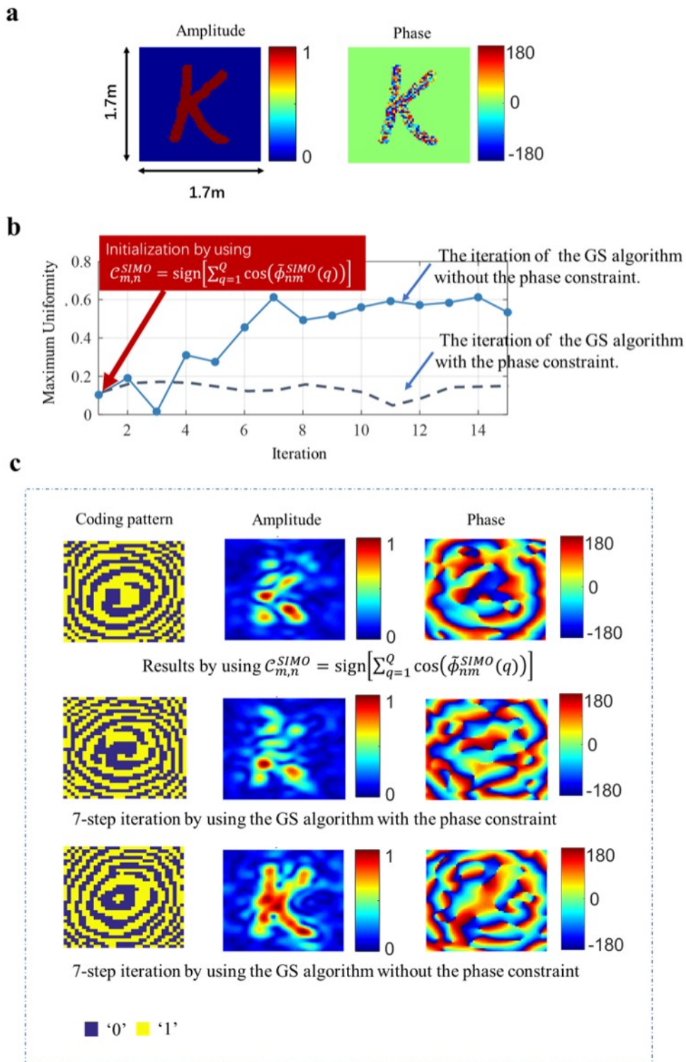
Figure 4 SIMO results for holographic imaging. The source is deployed at (0, 0, 2 \text{ m}) and the observation plane is at a distance of 3 \text{ m} from the one-bit coding metasurface. a . Amplitude (left) and phase (right) of the targeted hologram to be generated by the one-bit coding metasurface. b . Convergence of the GS algorithm with and without the phase constraint in terms of the maximum uniformity as figure of merit (see Eq. 1 in Ref. [53]). In both cases, the GS algorithm is initialized with c_{m,n}^{SIMO} = \text{sign}[\sum_{q=1}^Q \cos(\tilde{\phi}_{nm}^{SIMO}(q))] . c . Results using c_{m,n}^{SIMO} and Eq. 2 are shown in the top row, where the coding pattern of the one-bit metasurface, the amplitude and phase of the holographic image are shown on the left, middle and right, respectively. The corresponding results using the GS algorithm with and without the phase constraint are shown in the middle and bottom rows, respectively.
