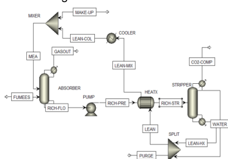
Figure 3a: Carbon capture without Heat Exchangers
