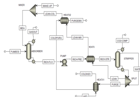
Figure 3b: Carbon capture with Heat Exchangers
