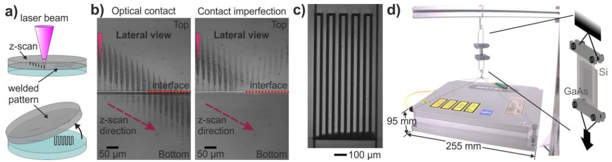
Fig. 1. a) Schematic representation of the welding procedure. b) Lateral view by IR transmission microscopy of the Si-Si interface. Imperfect contact leads to beam reflection at the interface and faulty welding. c) IR transmission image of a welded serpentine in the Si-GaAs configuration. Based on estimations the total welded area of \sim 0.25 \text{ mm}^2 should resist shear force up to 4.5 N. d) Image of the laser source used in the experiments ( \sim 3 \text{ kg} ) hanging from a Si wafer welded on GaAs. A schematic representation is shown on the right.
