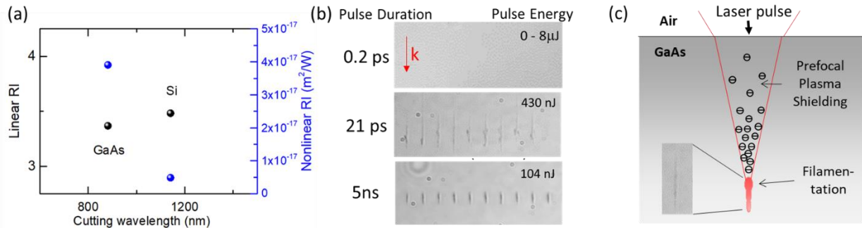
Fig. 1 (a) The comparison of material properties between GaAs and Si. RI represents refractive index. (b) The modification results of different pulse durations (NA=0.85). (c) Schematic of typical nonlinear effects that influence the laser focusing process inside GaAs. The inset shows the modification results corresponding to the filamentation regime.
