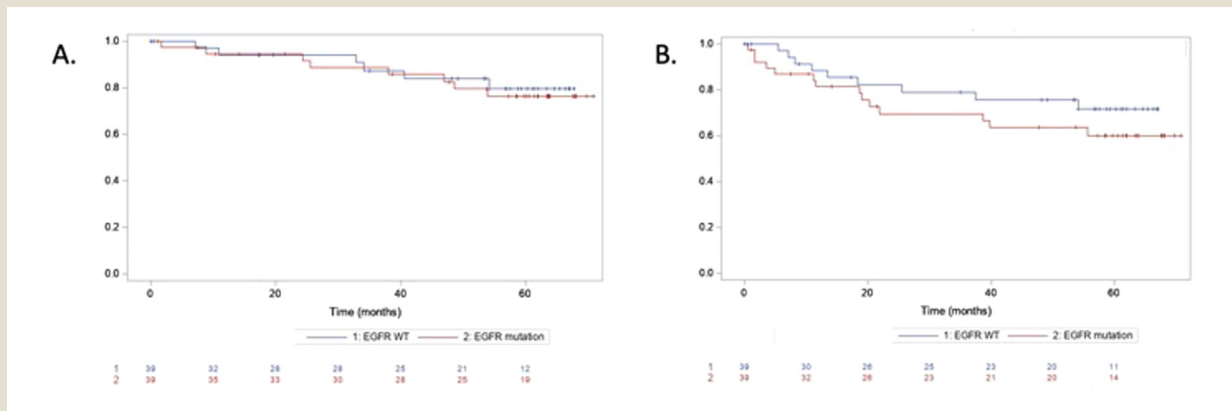
Figure 4 Kaplan-Meier Curves of the 78 Patients Included in the Matched groups (A) Overall survival (matched groups, n = 39 per group, P = .76 ); (B) disease-free survival (matched groups, n = 39 per group, P = .30 ).
