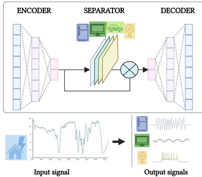
Fig. 1: Overview of Conv-NILM-net. It is composed of 2 blocs, the encoder/decoder and the separator. The encoder first projects the signal into a latent space, the separator disagggregates it into C corresponding to each appliance by learning C masks applied to input signal, then the decoder projects the C signals to the input space
