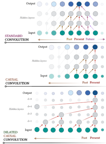
Fig. 2: Causal and dilated convolutions.
