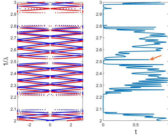
Figure 3. The functions \chi for a randomly perturbed medium. It is the same as that in fig. 2 with the width of the layers modified randomly with at most 1%. An edge mode is indicated by an arrow.
