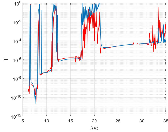
Figure 6. Transmission spectrum through the photonic crystal. In blue, the periodic structure, in red the random structure.
