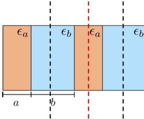
Figure 1. An example of stratified medium with inversion symmetry centers.
