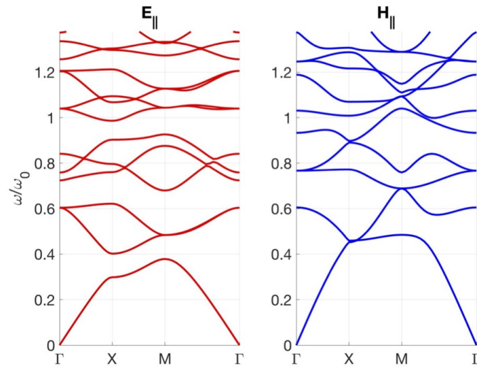
Figure 5. Band structure
