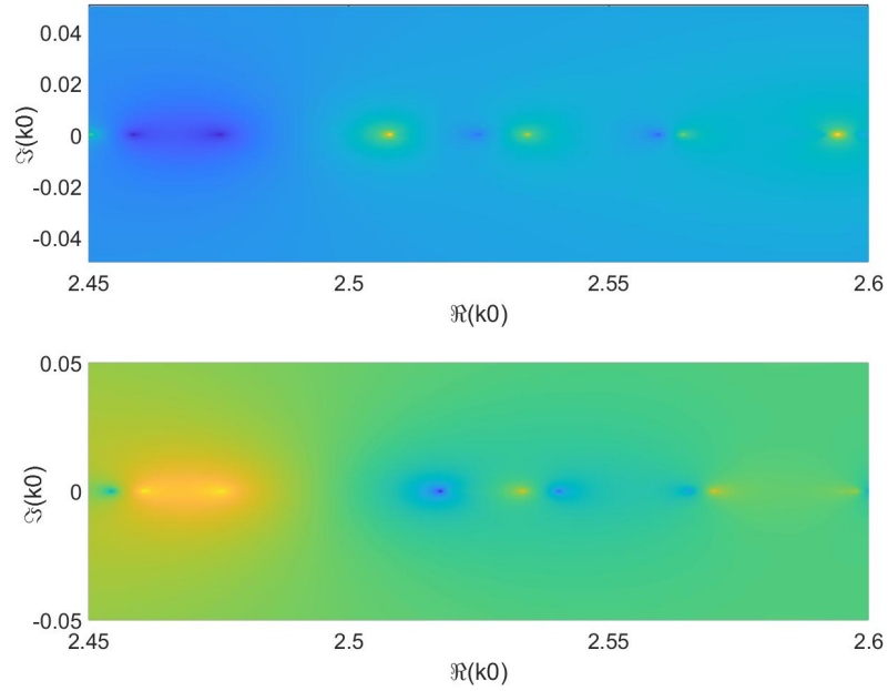
Figure 4. Pole and zero structure of the left and right photonic crystals in the presence of disorder. In the band gap between 2.5 and 2.55 the pole and zero are switched, which results in different topological classes.
