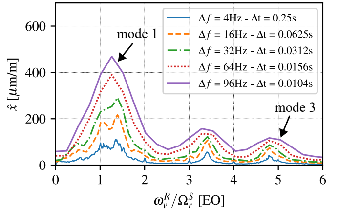
Fig. 5: FFT SPECTRA OF BLADE-MOUNTED STRAIN GAUGE FOR DIFFERENT BIN WIDTHS \Delta f
