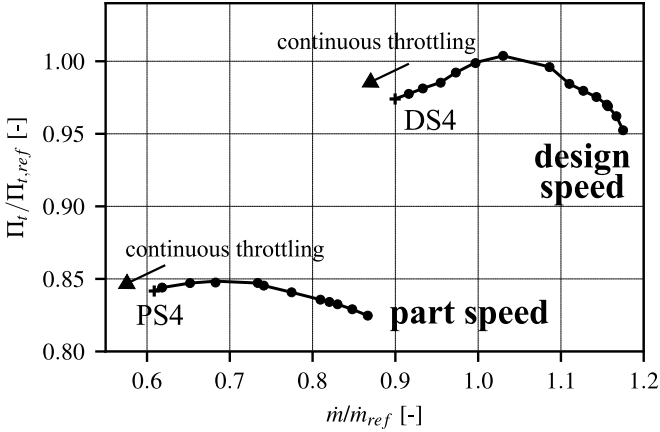
Fig. 3: FAN PERFORMANCE MAP AND INVESTIGATED OPERATING POINTS
