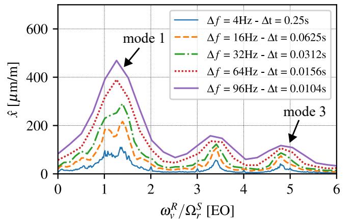
Fig. 8: RMS SPECTRA BASED ON PSD CALCULATION FOR DIFFERENT BIN WIDTHS \Delta f
