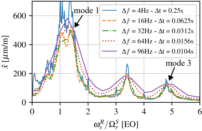
Fig. 14: CORRECTED FFT SPECTRA OF BLADE-MOUNTED STRAIN GAUGE FOR DIFFERENT BIN WIDTHS \Delta f
