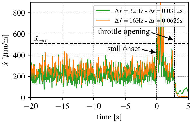
Fig. 16: CORRECTED AMPLITUDE OF FIRST EIGENMODE OVER TIME FOR DIFFERENT BIN WIDTHS \Delta f
