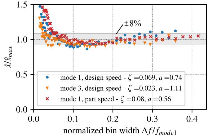
Fig. 15: CORRECTED MAXIMUM FFT AMPLITUDE AS A FUNCTION OF BIN WIDTH \Delta f
