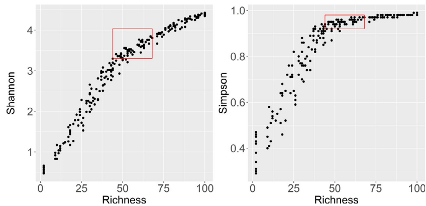
Figure 1. Distribution of calibration populations for Level-2 dataset along the Richness/Shannon or Richness/Simpson Index gradient. The range of diversity measured over Paracou is represented by the red box.
