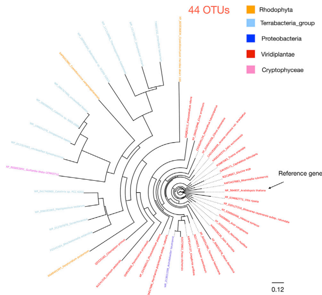
Figure 4. ClpS protein phylogeny after coarse tuning with Arabidopsis thaliana homolog as query
