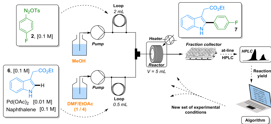
Scheme 2. Reaction setup for the optimization of indole 6 .
