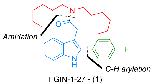
Fig. 1. Structure of FGIN-1-27 (1).
