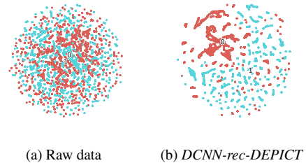
Fig. 3. Visualization with UMAP method of the dataset Orchards with the raw data and the latent space computed by the combination DCNN-rec-DEPICT . Blue is for traditional orchards and red for intensive orchards.
