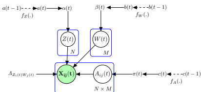
Fig. 1: Graphical representation of the Zero-Inflated dLBM model.
