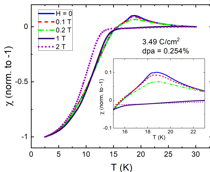
Figure 6. The magnetic-field dependence of TDR dynamic magnetic susceptibility in a 3.49 C/cm 2 electron irradiated sample. The indicated magnetic fields were applied parallel to c -axis. The inset zooms on the transition region.
