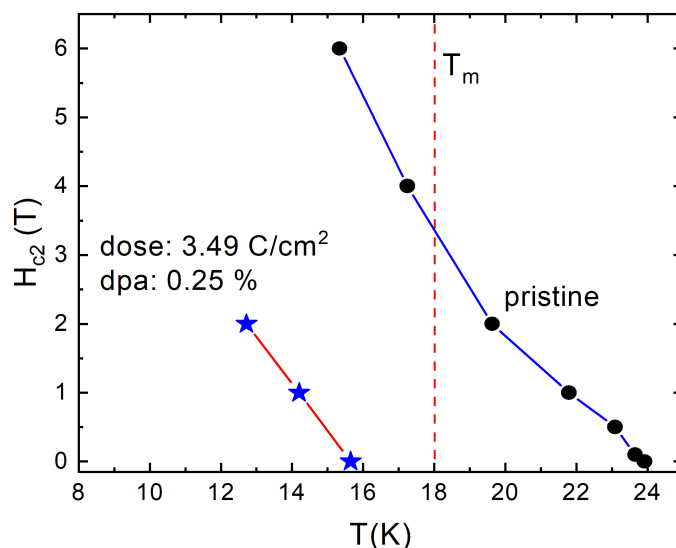
Figure 7. Upper critical field, H_{c2}(T) , of pristine (black circles) and 3.49 C/cm 2 electron irradiated (blue stars) \text{EuFe}_2(\text{As}_{0.77}\text{P}_{0.23})_2 with the magnetic field applied along the c -axis. Note that the slope, dH_{c2}(T)/dT near T_c in irradiated state is larger than the slope in the pristine state.
