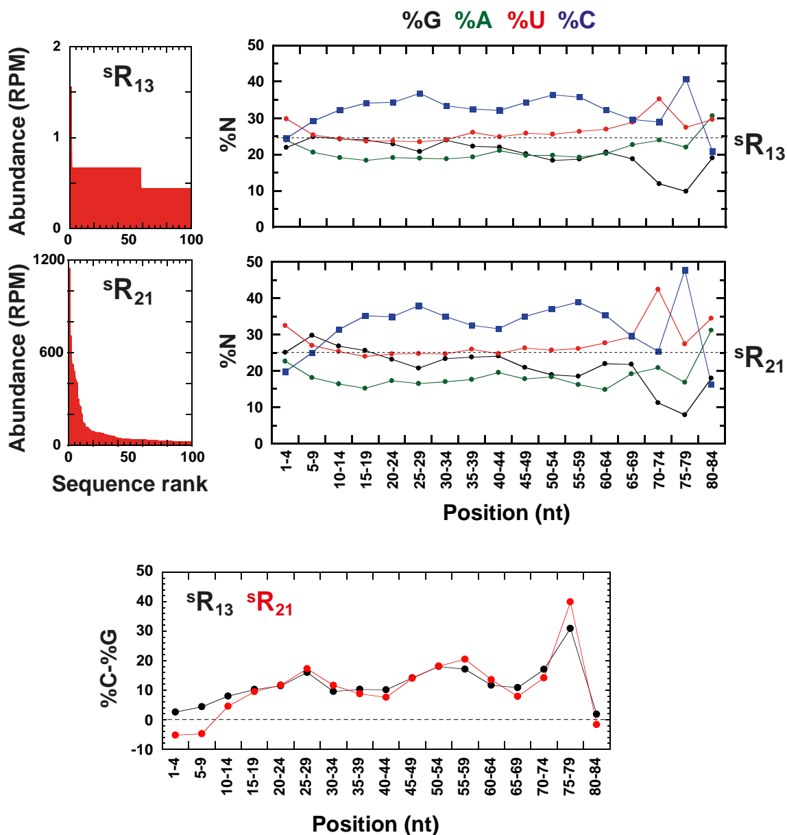
Figure S13: Compositions of the ^sR_{13} and ^sR_{21} sequence pools as determined by Illumina deep sequencing. The %N data were obtained by standard FastaQC analysis and thus represent the average %N per block of consecutive nucleotide residues along the N_{80} region for all sequences of the indicated library. Note the different scales on the abundance histograms indicating a much higher enrichment of the top-ranked sequences for the ^sR_{21} library.
