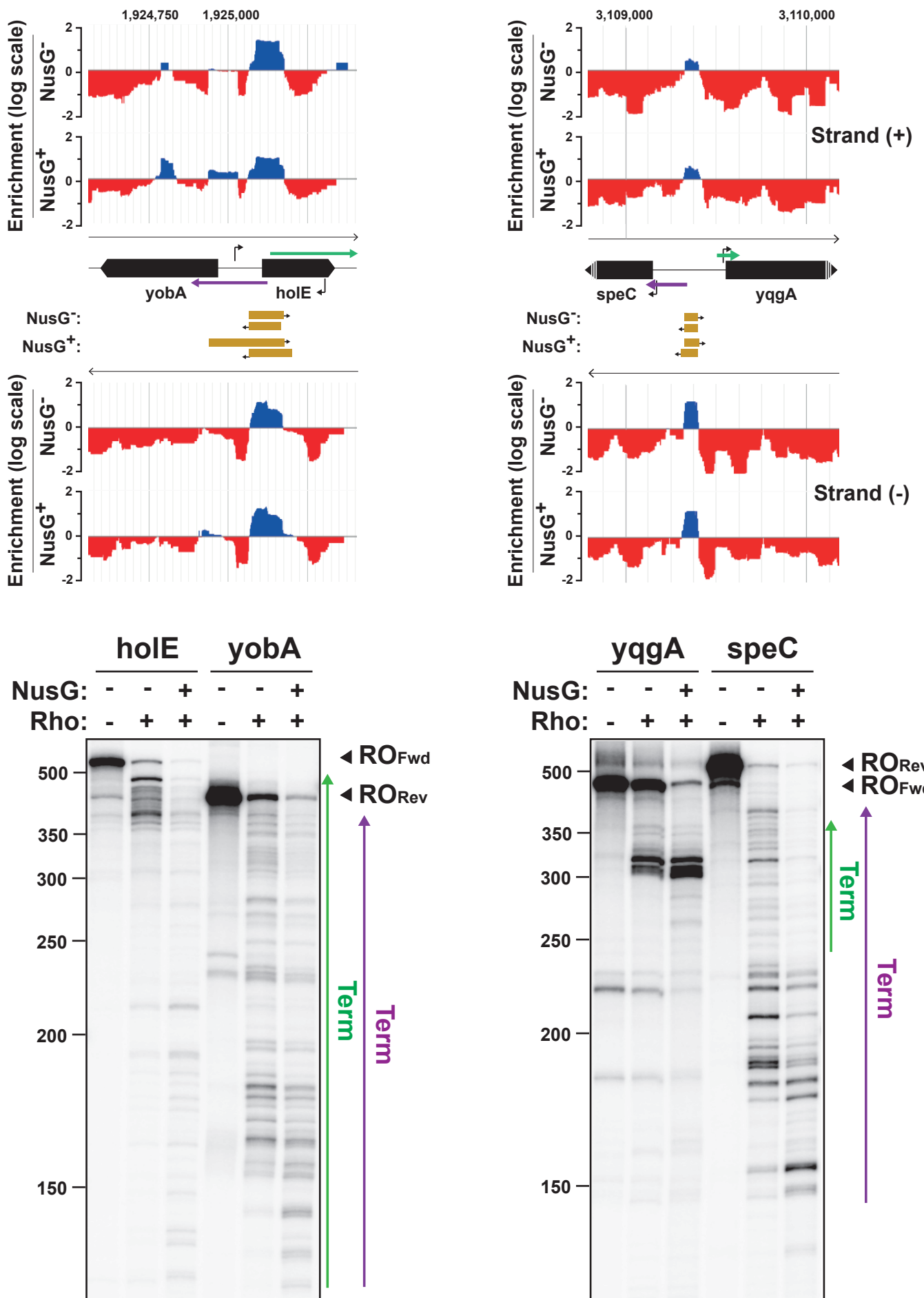
Figure S7: Representative examples of divergent Rut peak tandems (gold rectangles for peaks above the detection threshold, median \log_{10}FE \geq 0.3 ). Rho-dependent termination signals were confirmed by in vitro transcription termination experiments with DNA templates hoIE, yobA, yqgA, and speC (see Table S5 for details). Green and purple arrows indicate the termination regions observed in the forward (strand +) and reverse (strand -) directions, respectively. 'RO' and 'Term' locate runoff and termination transcript bands, respectively. Different x-axis scales are used for the left and right diagrams.
