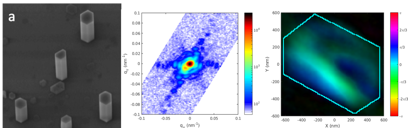
Figure 1. Left: electron microscopy of a typical area of the sample. Centre: (HK0) slice through the reciprocal space map around the (115) forbidden reflection. Right: 2D image of the complex scattering function in the basal plane as obtained from phase retrieval (the modulus and the phase are encoded by the brightness and the colour, respectively). The bright hexagon is a guide to the eye.
