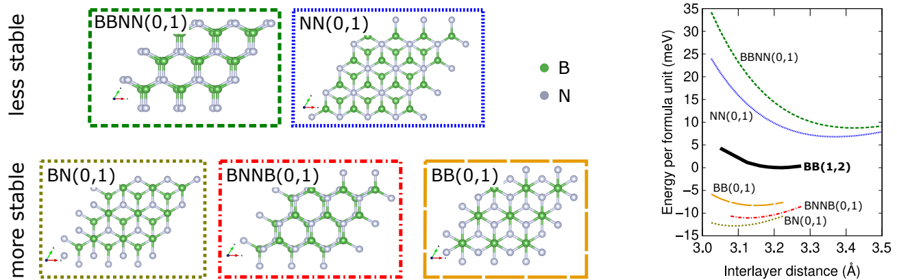
FIG. 10. The five hexagonal stackings in untwisted bilayers and their stability curves with respect to the BB(1,2) twisted bilayer (thick black solid line).
