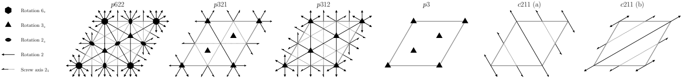
FIG. 7. All the possible layer groups of the moiré bilayer graphene and h-BN periodic structures (adapted from [34], see text). The trivial group p1 is not shown.
