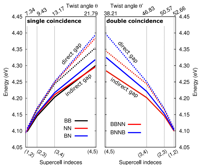
FIG. 5. Indirect gap (solid lines) and lowest direct transition (dashed lines) of the five stackings as a function of the twist angle ( \theta or \theta' depending on the stacking) within the \delta = 1 family.
