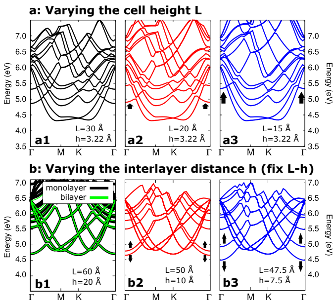
FIG. 11. The evolution of the NFE states as a function of the simulation parameters in the BN(1,2) bilayer. a : evolution as a function of the cell height L at fixed interlayer distance ( h = 3.22 \text{ \AA} ). L = 30, 20 and 15 \text{ \AA} in panels a1 , a2 and a3 respectively. b : evolution as a function of the interlayer distance h at fixed vacuum ( L - h = 40 \text{ \AA} ). h = 20, 10 and 7.5 \text{ \AA} in panels b1 , b2 and b3 respectively. In panel b1 , the band structure of the BN(1,2) bilayer (flashy green) is compared with that of the isolated monolayer (black).
