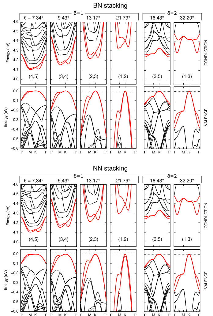
FIG. 4. Bottom conduction and top valence of the BN and NN stackings at different twist angles.
