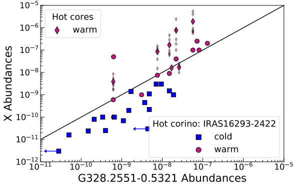
Fig. 18. Molecular abundances relative to \text{H}_2 towards IRAS 16293–2422 (Schöier et al. 2002; Maret et al. 2005; Jaber et al. 2014; Taquet et al. 2014; Majumdar et al. 2016) and hot cores from Bisschop et al. (2007) vs. that of G328.2551-0.5321. The diamond represents the COMs in the hot cores. The small symbols are used to show each hot core. The larger symbol shows the averaged value. The blue data points represent the cold component of the envelope, and red represents the warm component of the envelope. The grey shaded region corresponds to a factor of 5 scatter from the one-to-one relation.
