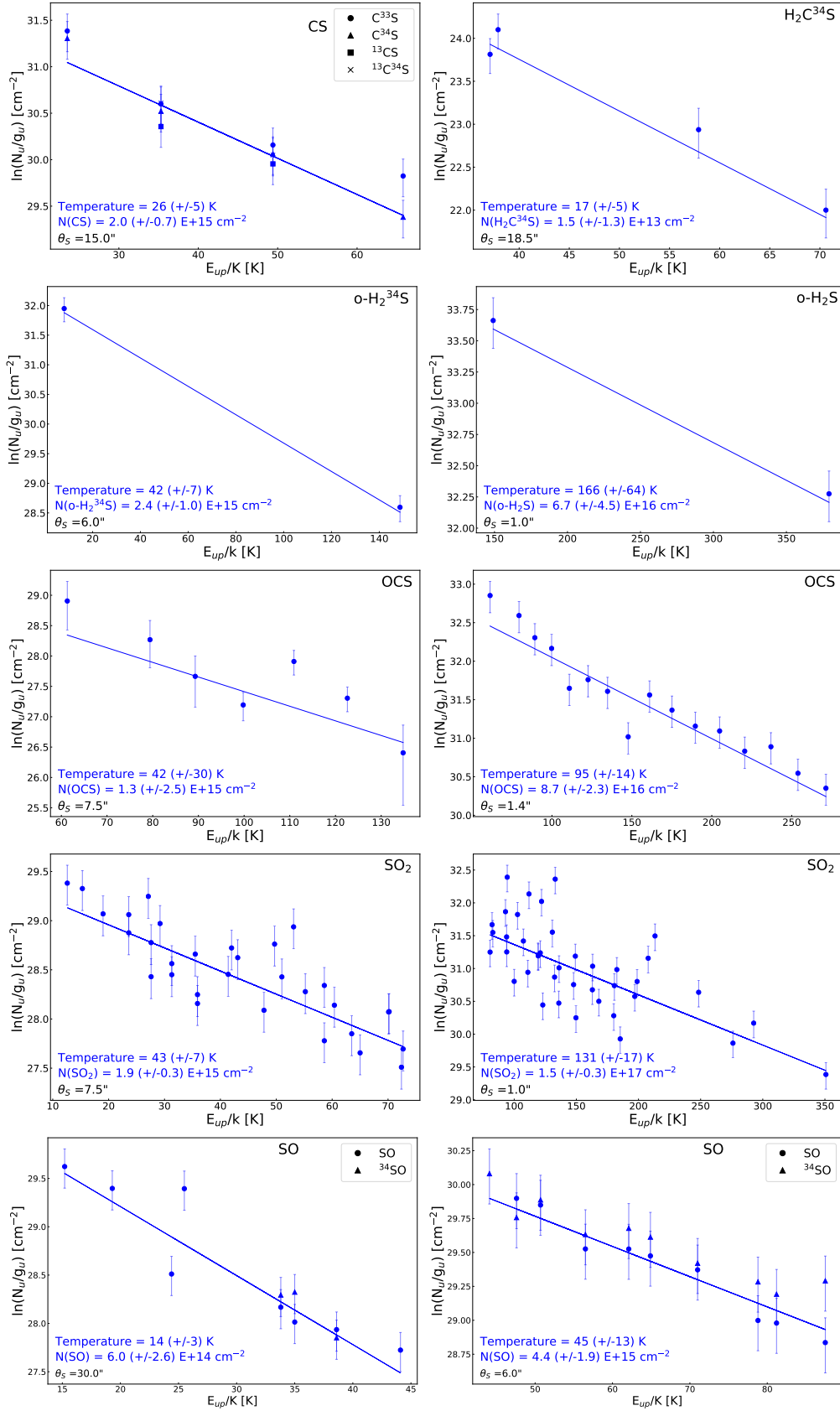
Fig. B.4: Rotational diagrams of the S-bearing molecules CS, \text{H}_2^{34}\text{S} , ortho- \text{H}_2\text{S} , OCS, \text{SO}_2 , and SO. The emission from the cold component of the envelope for \text{H}_2\text{S} is described by the rotational diagram of o- \text{H}_2^{34}\text{S} . The two rotational diagrams of OCS, \text{SO}_2 , and SO represent the narrow and the broader components of the Gaussian fit.
