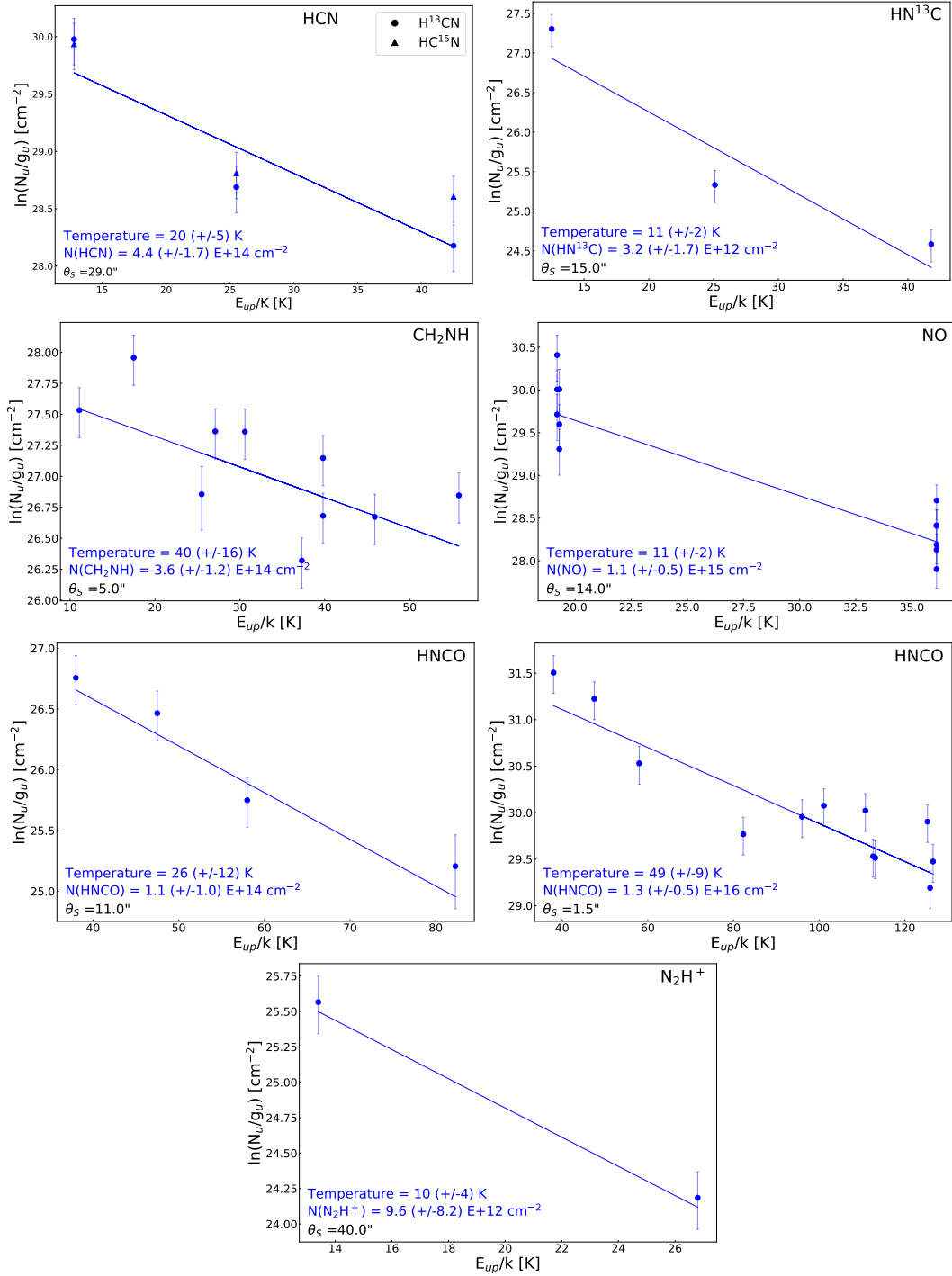
Fig. B.3: Rotational diagrams of the N-bearing molecules HCN, HN 13 C, CH 2 NH, NO, HNC0, and N 2 H + . The two rotational diagrams of HNC0 represent the narrow and the broader components of the Gaussian fit.
