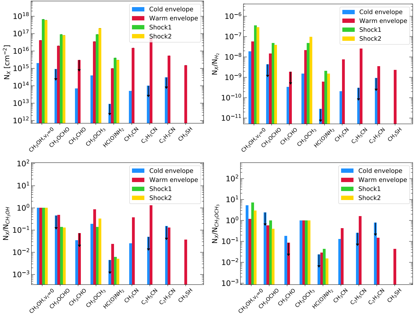
Fig. 17. COM column densities ( top left panel ) and abundances relative to H_2 ( top right panel ), methanol ( bottom left panel ) and dimethyl ether ( bottom right panel ). Only the main isotopologues are represented. The cold and warm components of the envelope are described by the blue and red histograms. The two shocks are represented in yellow and green. The upper limits are indicated by the black arrows.
