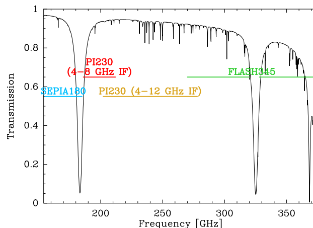
Fig. 1. Continuous frequency coverage of the spectral survey. The black curve shows the atmospheric transmission as computed by the ATM model written by Juan Pardo ( Pardo et al. 2002 ) with a water vapour of 1.2 mm.
