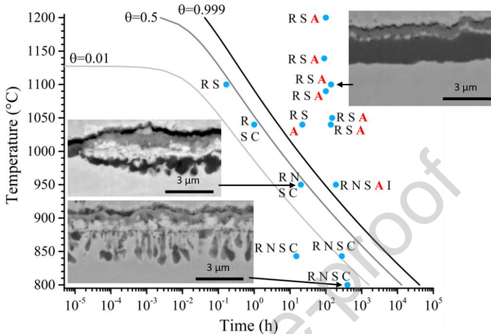
Fig. 12. Time-temperature- \theta diagram. Dots represent isothermal oxidation and letters represent the oxide identified by XRD after oxidation (R = rutile, S = spinel, A = Al 2 O 3 , C = Cr 2 O 3 , N = NiO, I = ilmenite). Lines represent the different values of \theta calculated with the model.
