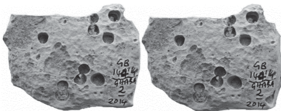
Figure 3. GB 144'14, stereo images of lithophage borings in limestone from locality GB 2.
