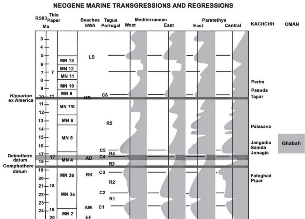
Figure 40. Eustatic history of the Mediterranean and Paratethys, the Tagus succession (Portugal) and Southwestern Africa, with major biostratigraphically significant faunal dispersal events (proboscideans and equids) and correlations of fossiliferous deposits in Oman and Kachchh (India). (Abbreviations - RS83 : Rögl & Steininger (1983), MN : Mammal Neogene zones of Europe, AD : Arrisdraft, AM : Auchas Main, EF : Elisabethfeld, HB : Hondeklip Bay, LB : Langebaanweg; RK : Ryskop, C : Transgression Cycle Tagus, R : Regression Cycle Tagus, Ma : Mega-annum) (modified from Bhandari et al. 2015)
